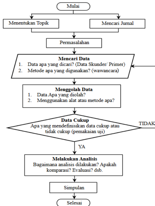
Gambar 3.3 Contoh Flowchart
